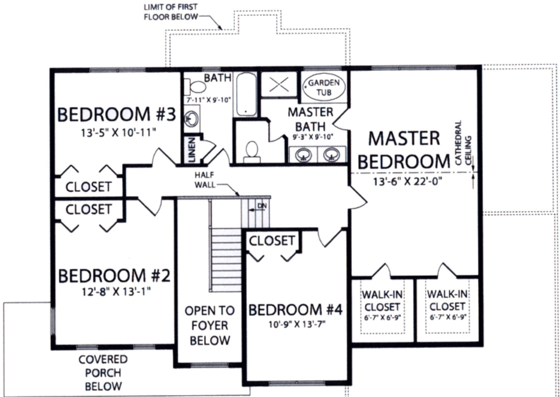
THE HAMILTON SECOND FLOOR PLAN
